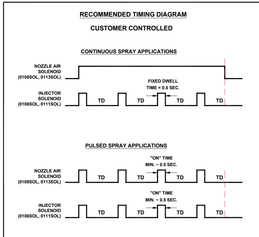
Fig. 1: Timing configuration for VS Manifold Assembly
