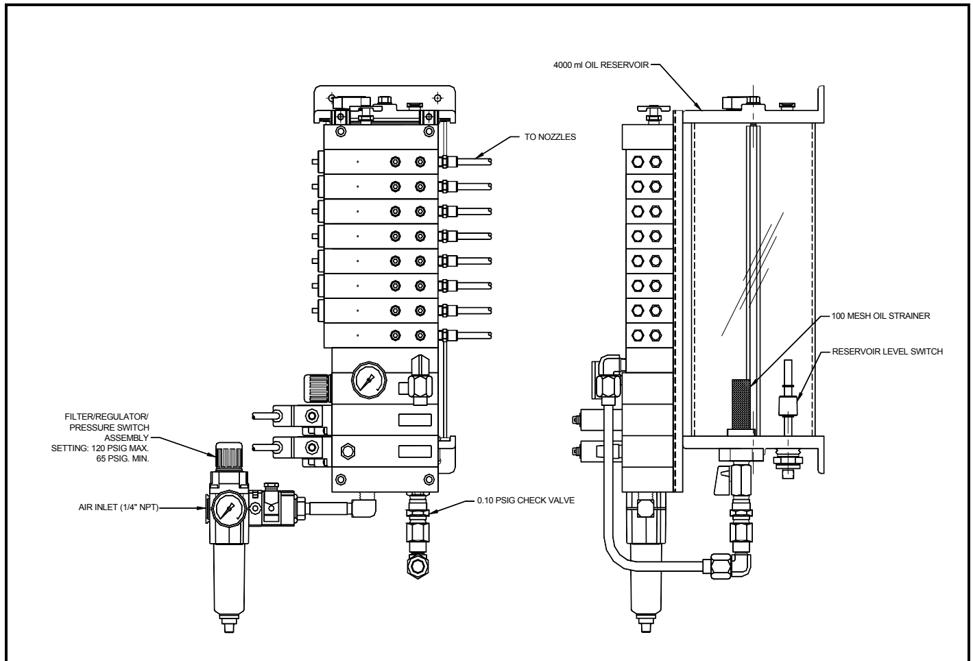
Fig. 5: VSR Assembly w/ Manual Fill Reservoir and VS Manifold assembly with Eight Injectors
