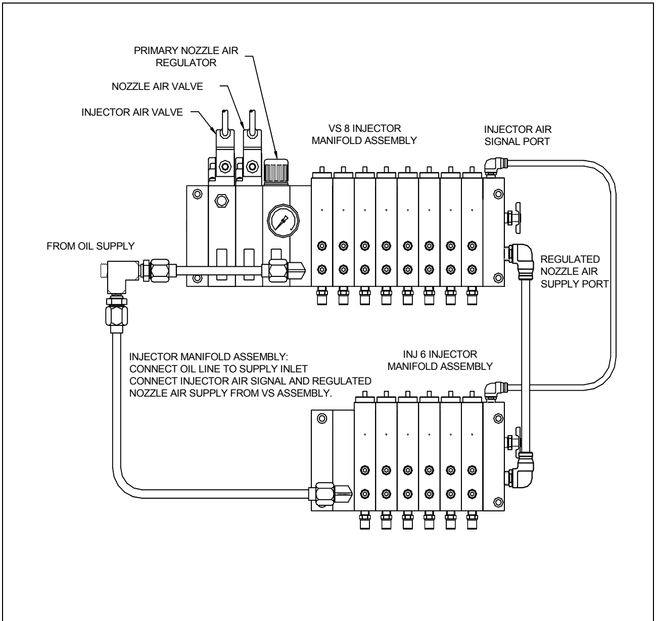
Fig. 4: VS Manifold Single network, Single Regulator Assembly with Eight Injectors INJ Manifold Assembly with Six Injectors
