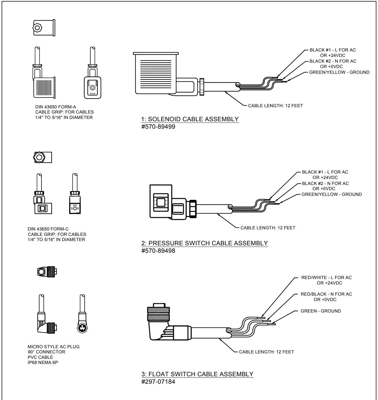
Fig. 6: VS/VSR Cable Assemblies
